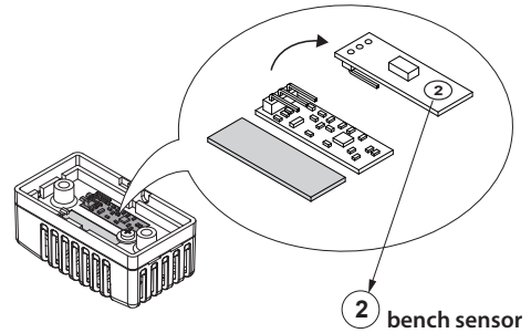
2 bench sensor
