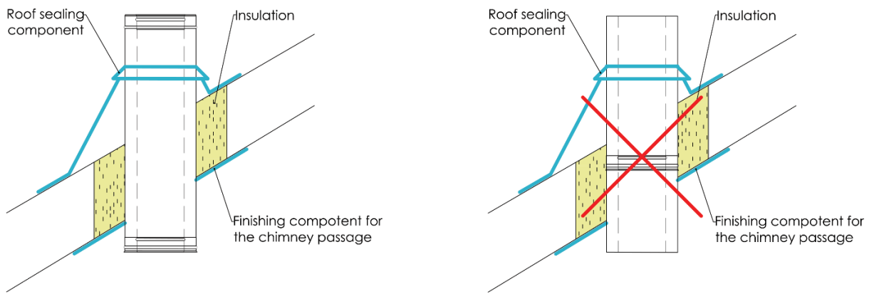
Fig.4. Mounting of the chimney system in the places of intersection with the building structure
