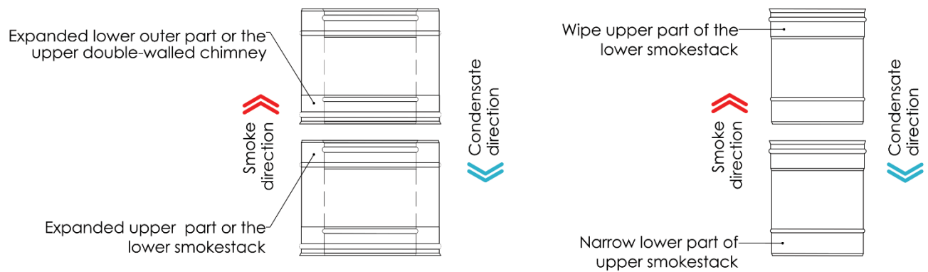
Fig.3.Assembling of the double-walled chimney
